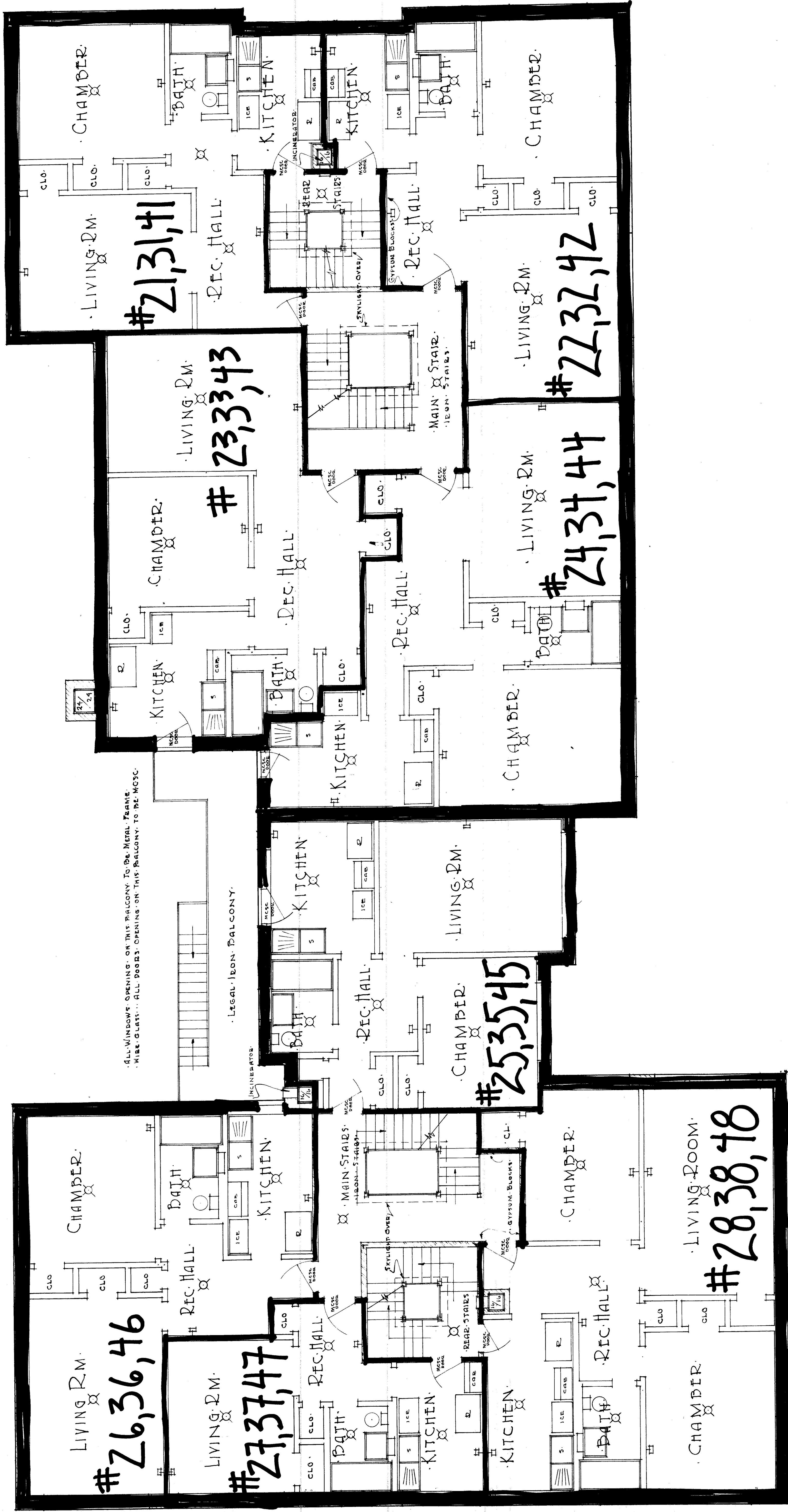
TYPICAL FLOOR PLAN.
